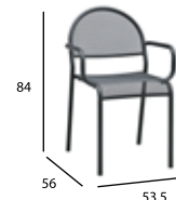
Armchair Steel Ref. AniAch Stackable: yes 5.8 Kg
